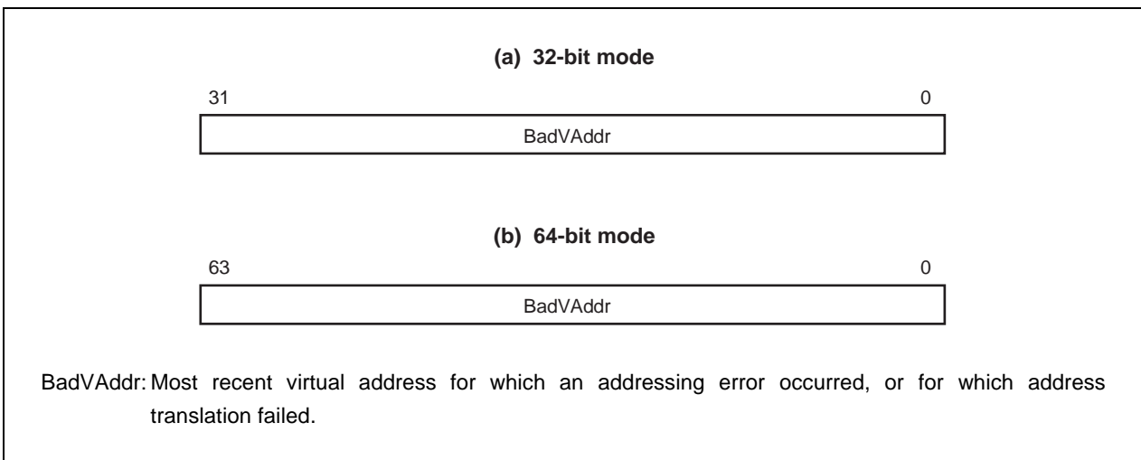
Figure 3-8. BadVAddr Register
