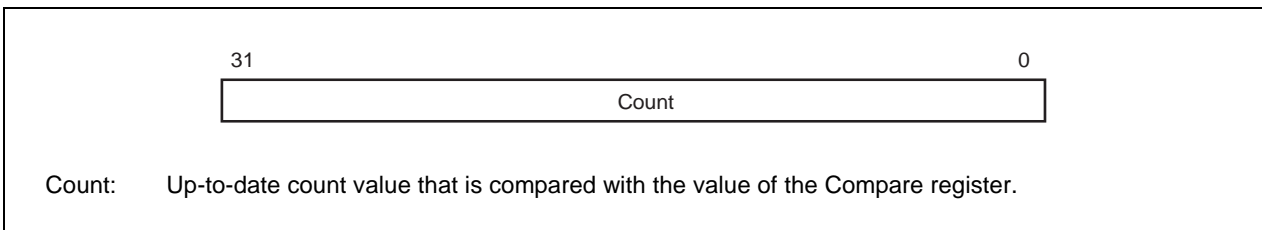
Figure 3-9. Count Register
