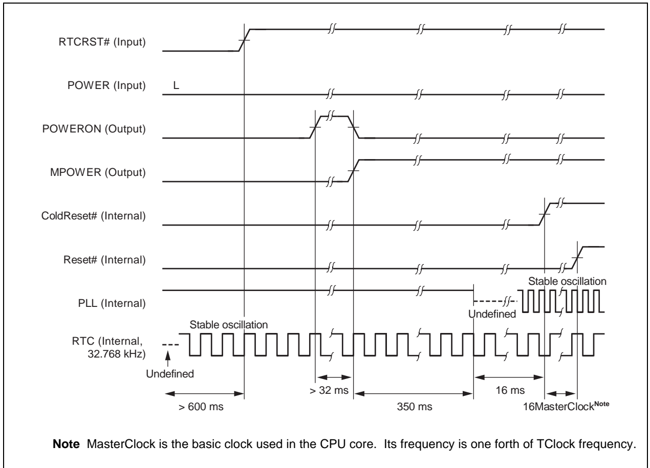
Figure 5-1. RTC Reset
