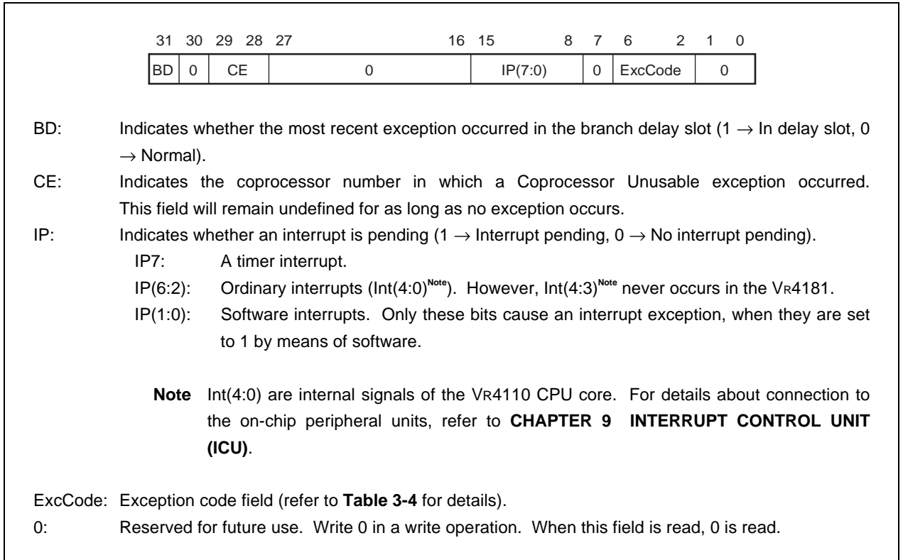
Figure 3-14. Cause Register
