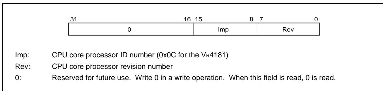
Figure 3-17. PRId Register
