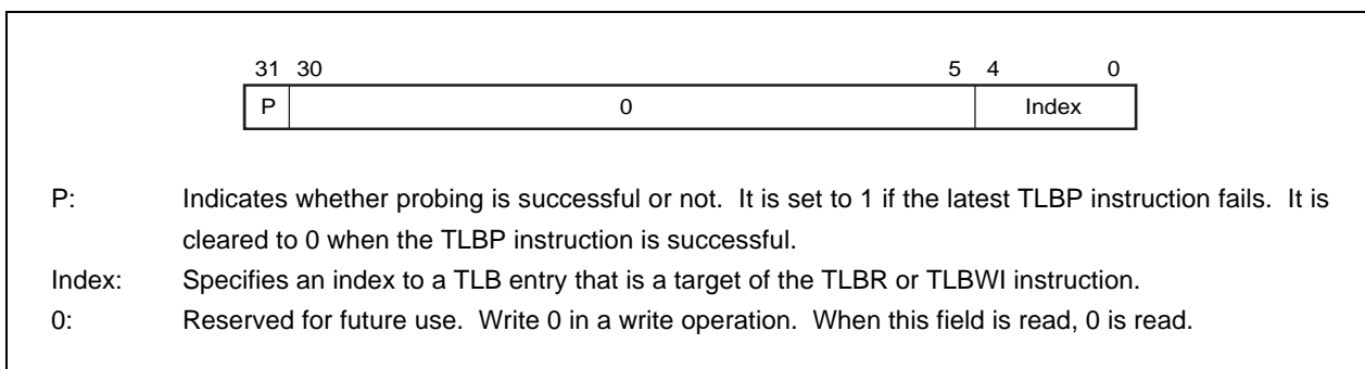
Figure 3-1. Index Register
