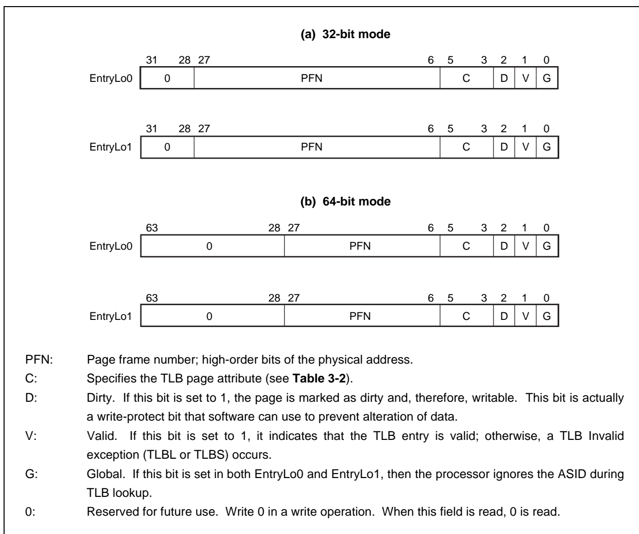
Figure 3-3. EntryLo0 and EntryLo1 Registers
