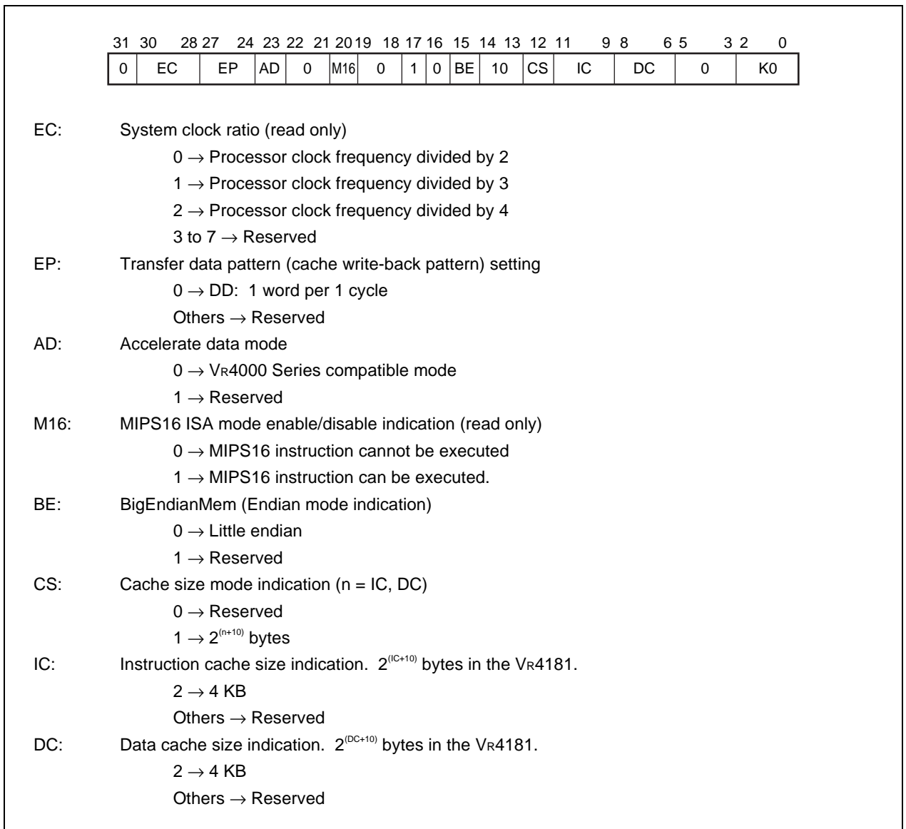
Figure 3-18. Config Register (1/2)
